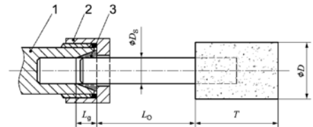
Fig. 1: Clamping length of chuck and collet Key
